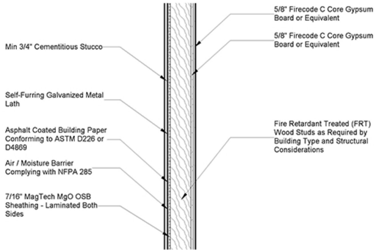
① CF/WPPS 120-02 - Section (Typ.) 3/4" = 1'-0"
